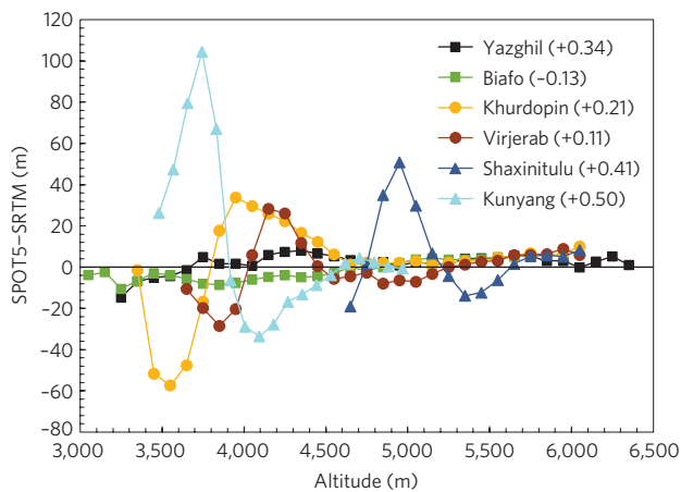
Figure 3 | Elevation changes with altitude between February 2000 and December 2008 for selected surge-type and non-surge glaciers. We plotted: two glaciers that surged between 2000 and 2008 (triangles); two glaciers in their quiescent phase between 2000 and 2008 that surged before 2000 (circles); and two non-surge glaciers (squares). Error bars are not shown for clarity but range between \pm 0.25 m and \pm 17.24 m (mean error of \pm 2.72 m). The location of each glacier is given in Fig. 1. Numbers in the legend correspond to the glacier-wide mass balances ( \text{m yr}^{-1} w.e.).
